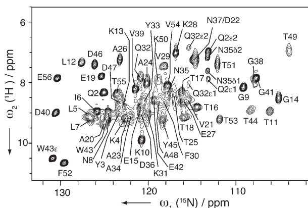
Figure 1. Solid-state ^1\text{H} -detected ^{15}\text{N} – ^1\text{H} 2D NMR spectrum of uniformly- ^{13}\text{C} , ^{15}\text{N} , ^2\text{H} -labeled GB1, back-exchanged with ^1\text{H}_2\text{O} (750 MHz, 39 kHz MAS, 2 s recycle delay, 2 scans per row, t_1^{\text{max}}(^{15}\text{N}) = 50 ms, t_2^{\text{max}}(^1\text{H}) = 30 ms, total 30 min). No apodization or post-acquisition solvent suppression was applied. Assignments were derived from 3D experiments.
